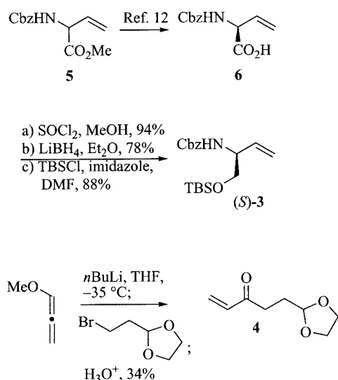
Scheme 2. Synthesis of CM partners.
