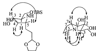
Figure 2. Correlation observed in the nOe spectra of pyrrolidine 8 and hyacinthacine A 2 .
