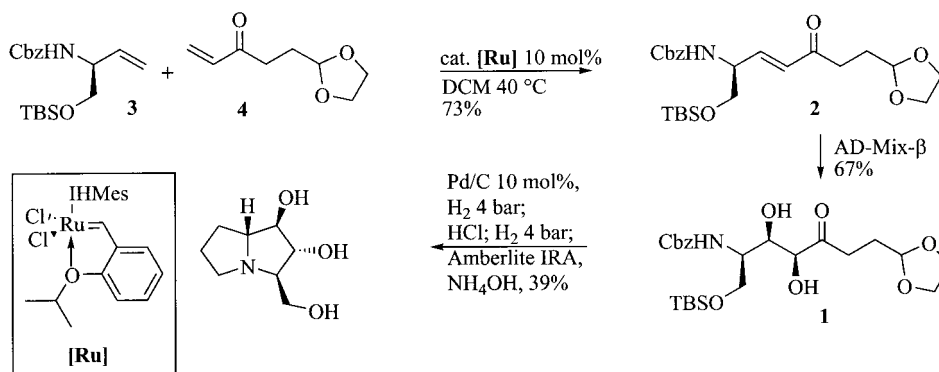
Scheme 3. Synthesis of hyacinthacine A 2 [IHMEs = 1,3-bis(2,4,6-trimethylphenyl)-4,5-dihydroimidazol-2-ylidene].
