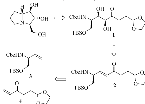
Scheme 1. Retrosynthetic analysis of hyacinthacine A 2 .
