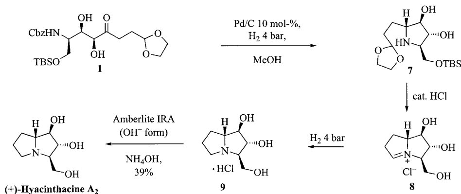
Scheme 4. Sequential double reductive cyclization.
